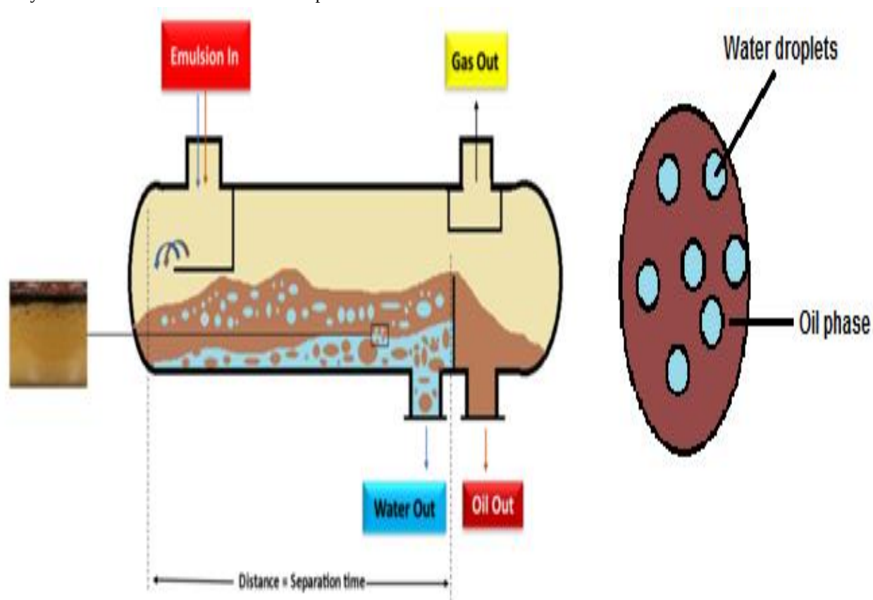
Figure 10: The above Figure Represents Emulsion in Separator.
