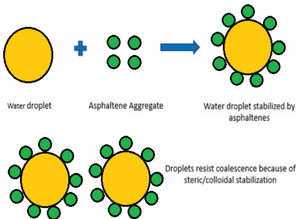
Figure 11: Illustrates the Mechanism of Emulsion Stabilization by Asphaltenes.
