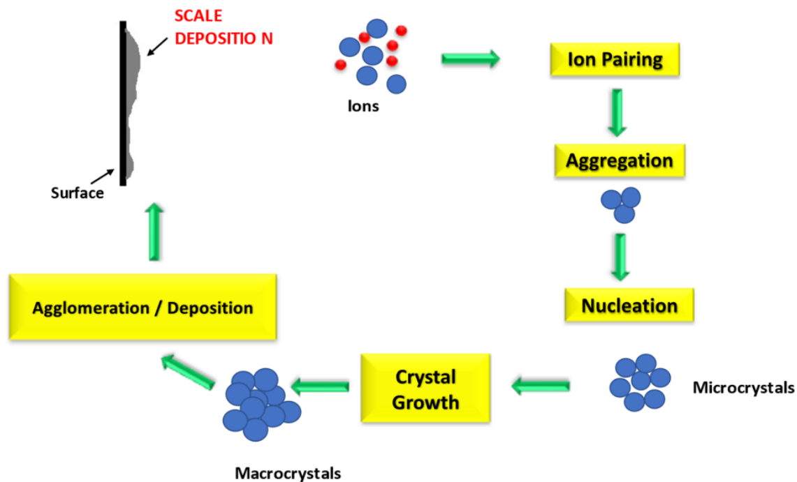
Figure 7: Illustrates the Mechanism of scale formation.
