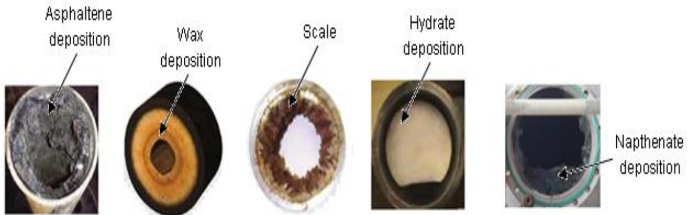
Figure 2: The above Figure Represent the Solid Deposition in Pipeline.
