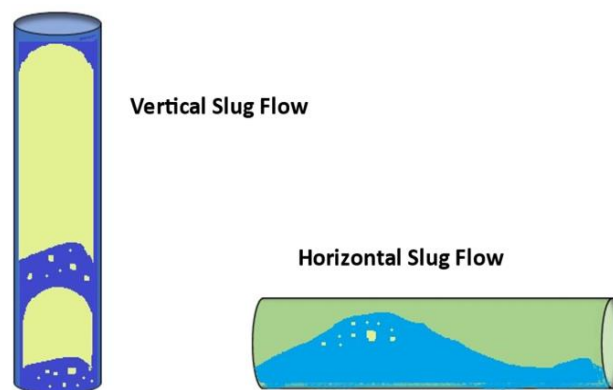
Figure 6: The above Figure Shows the Slug Flow in the Pipeline.
